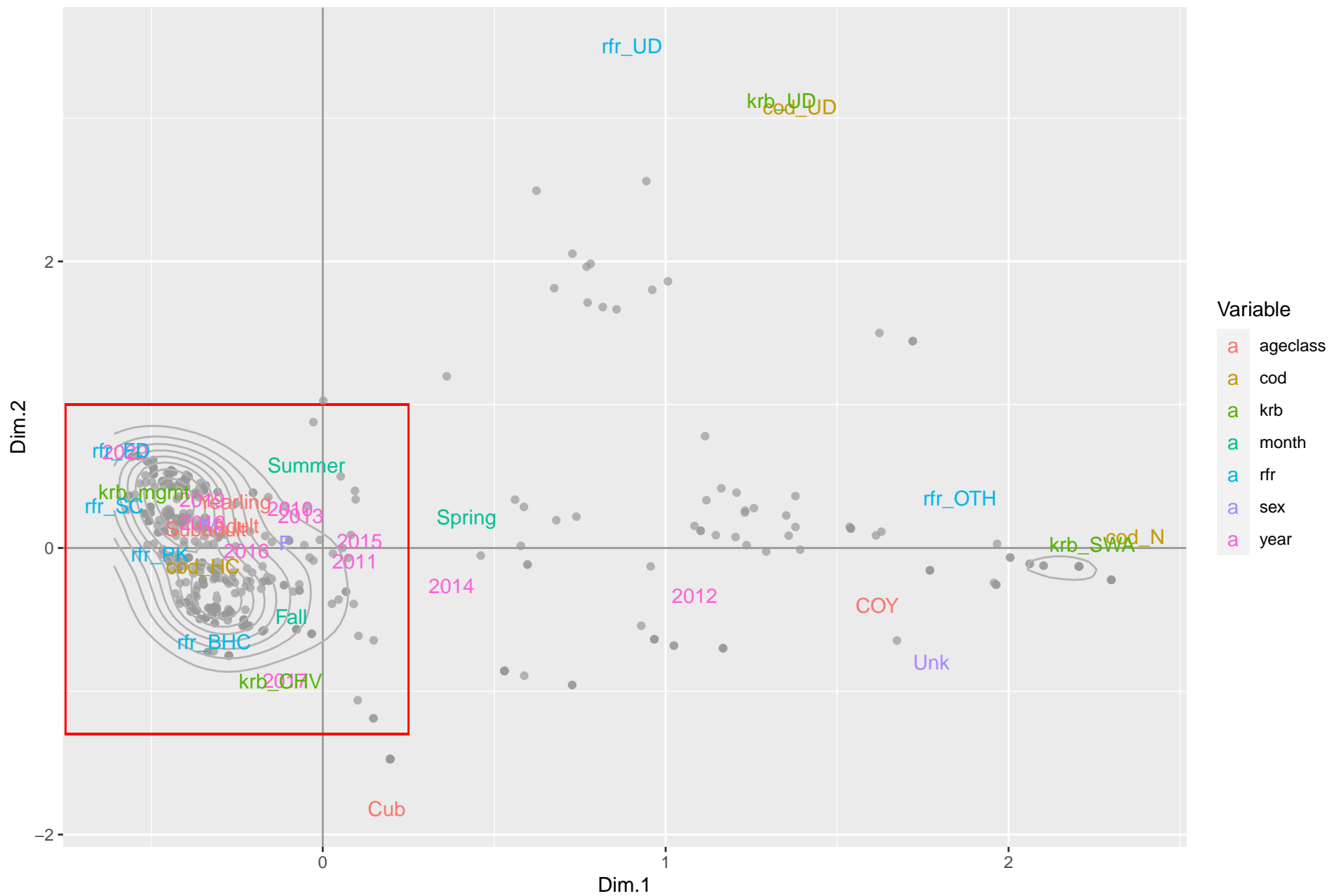
MCA Plot of the Grizzly Bear Data
