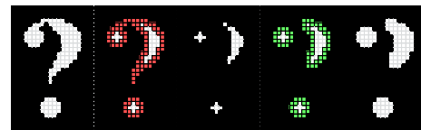
Figure 6: Opening: Left: Original Image. Second from Left: Erosion Marked. Center: Results of Erosion. Second from Right: Dilation Marked. Right: Results of Dilation (Opening Complete).
