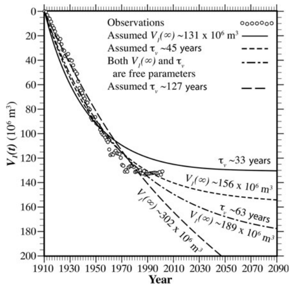
Fig. 5. Observed or estimated variations in ice volume for Storglaciären fitted to an equation of the form V_i(t) = V_i(\infty) \times (1 - e^{-t/\tau_v}) . The different curves correspond to different assumptions made regarding the value of V_i(\infty) or \tau_v given in the explanation; curves are labeled according to estimated parameters (see text for discussion).
