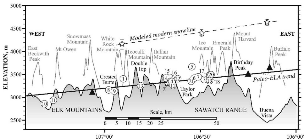
FIGURE 6. LGM and model-simulated modern ELA trends along an east–west cross section through study area. Numbers in circled points correspond to the paleoglaciers identified in Figure 2, triangles are LGM ELAs reported by Leonard (1989), and stars are estimates of modern ELAs with model uncertainties shown. Topography is generalized, and individual peaks are shown to convey the terrain in the study area.
